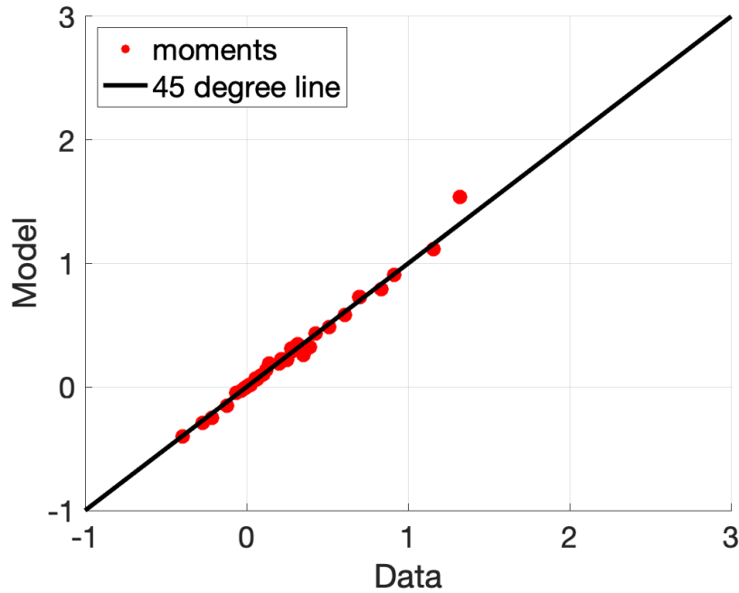
Figure C.1: Model Fit
